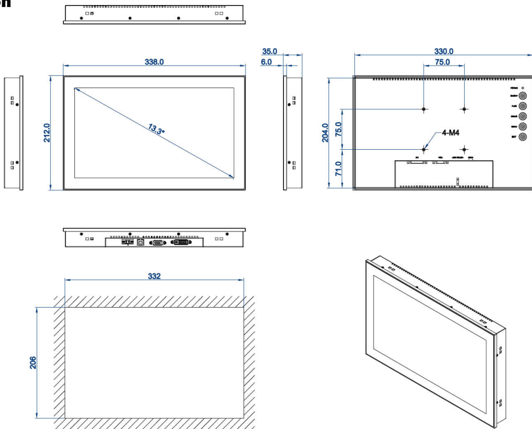
DIMENSIONAL DRAWING:TM-DPC133
