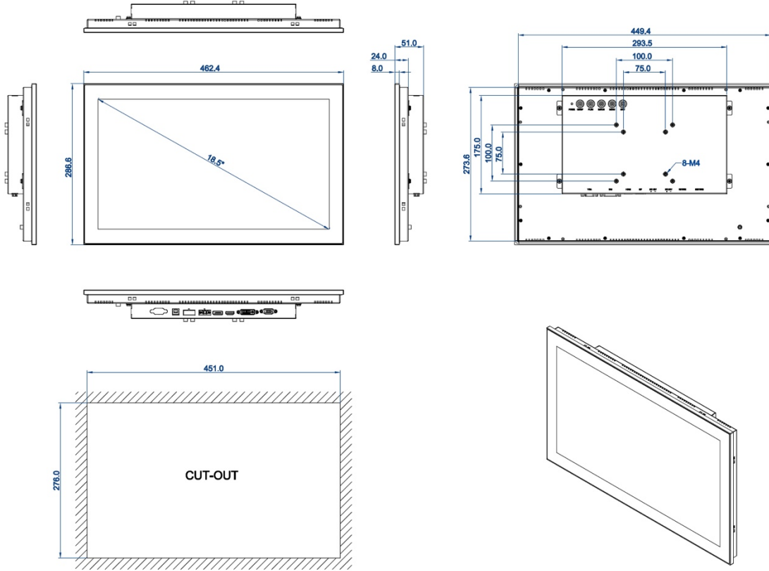
DIMENSIONAL DRAWING:TM-PCA185
