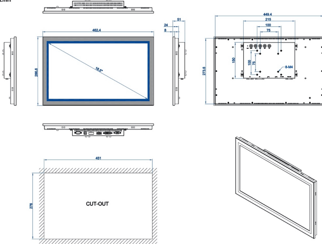
DIMENSIONAL DRAWING:TM-PR185
