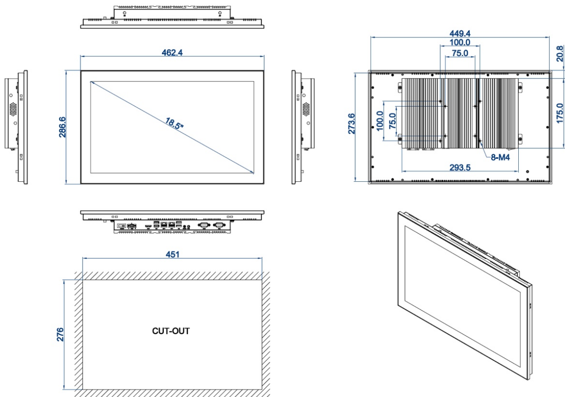
DIMENSIONAL DRAWING:TPC-DCM185
