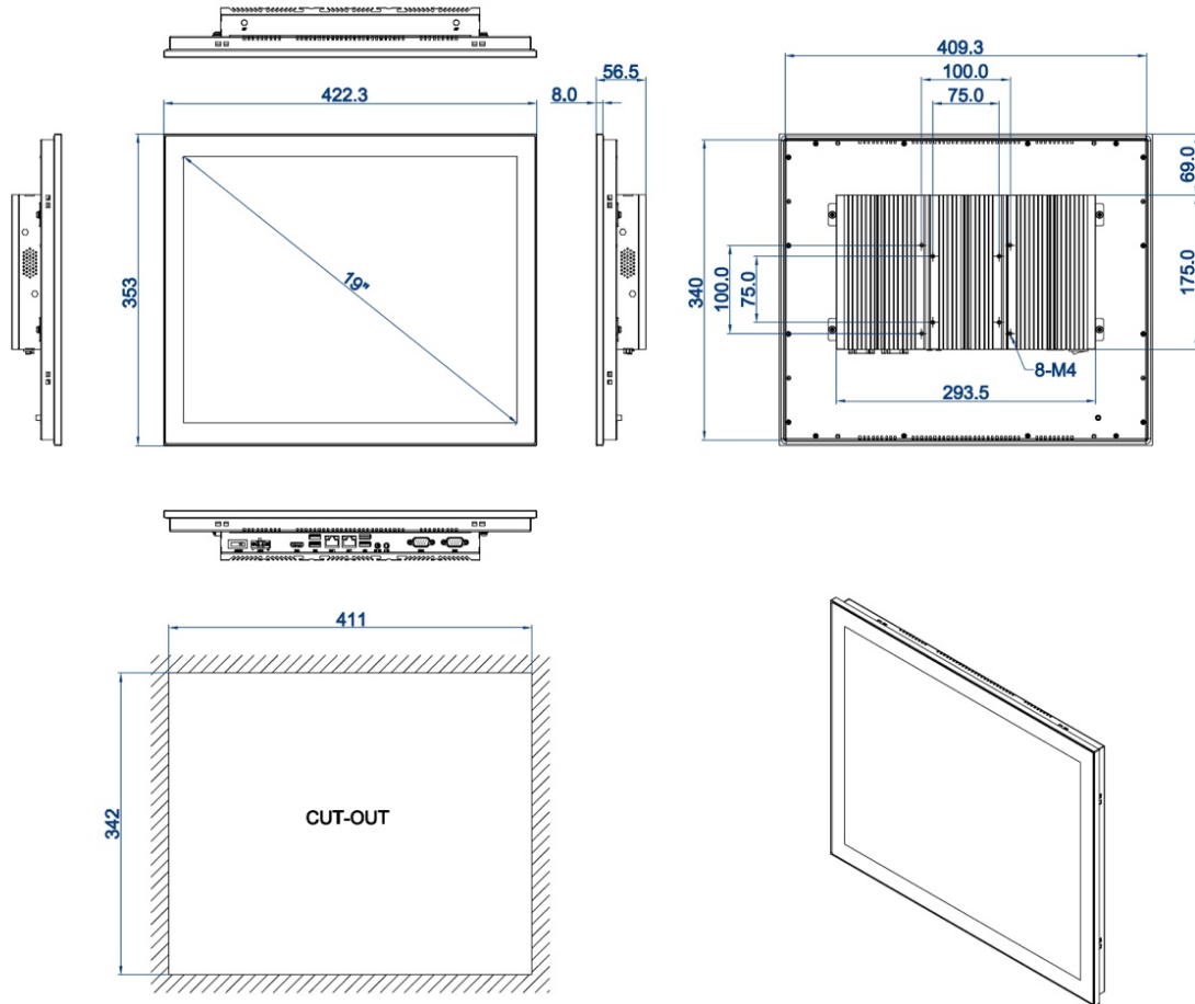
DIMENSIONAL DRAWING:TPC-DCM190
