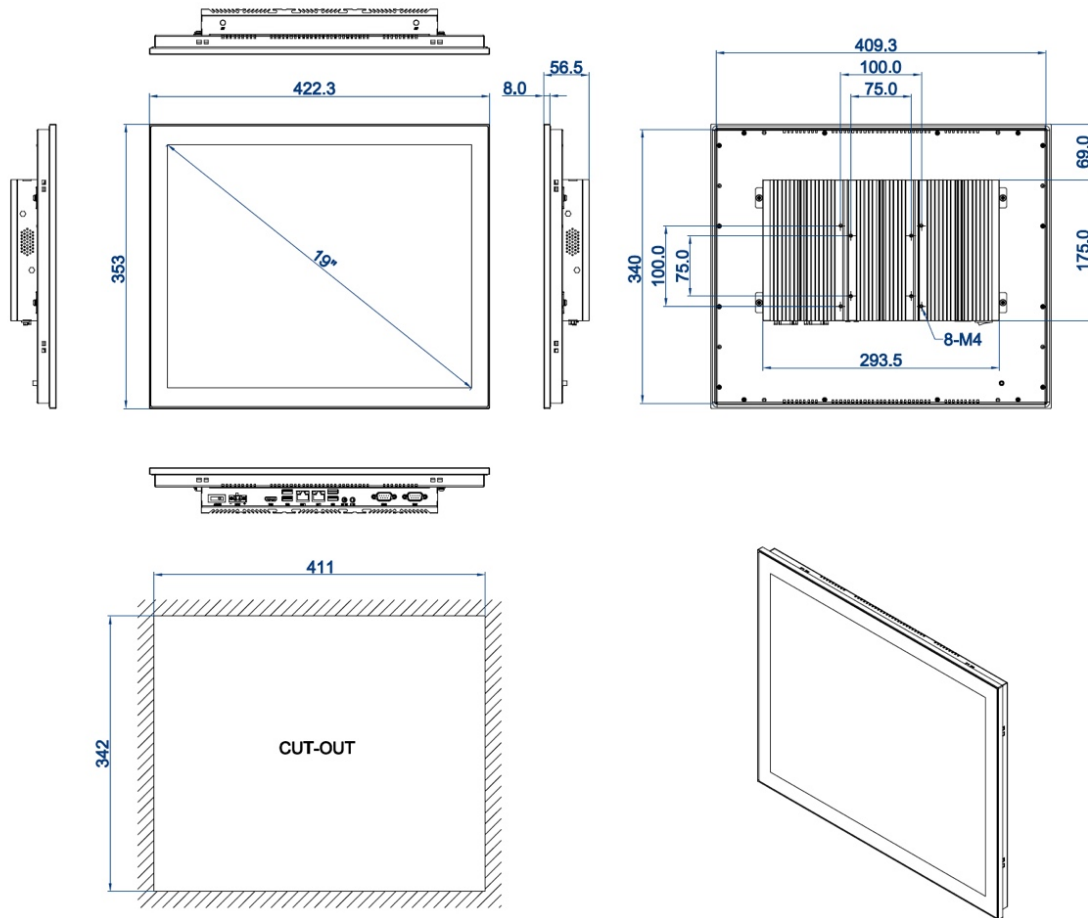
DIMENSIONAL DRAWING:TPC-DCM190
