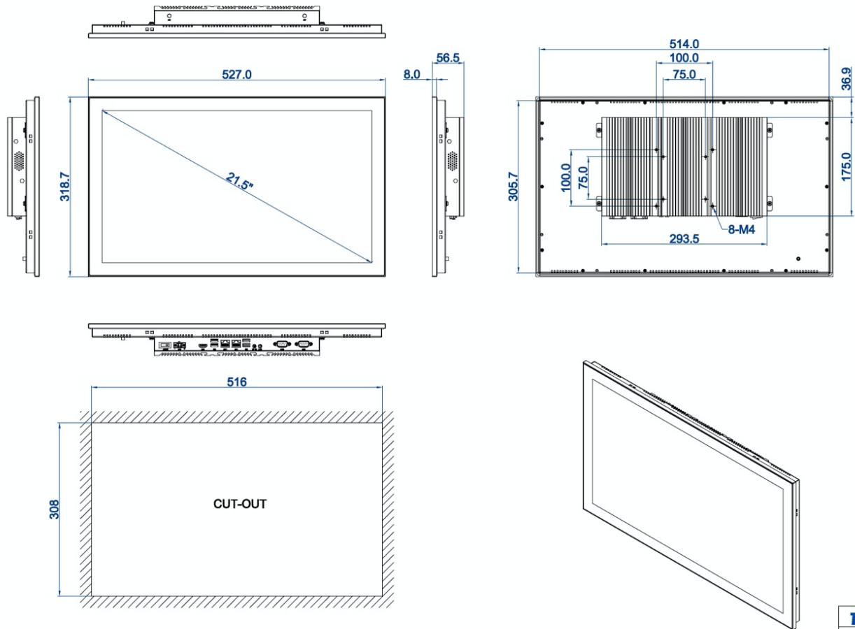
DIMENSIONAL DRAWING:TPC-DCM215
