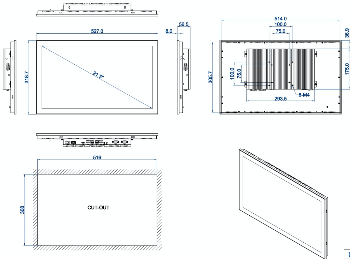
DIMENSIONAL DRAWING:TPC-DCM215
