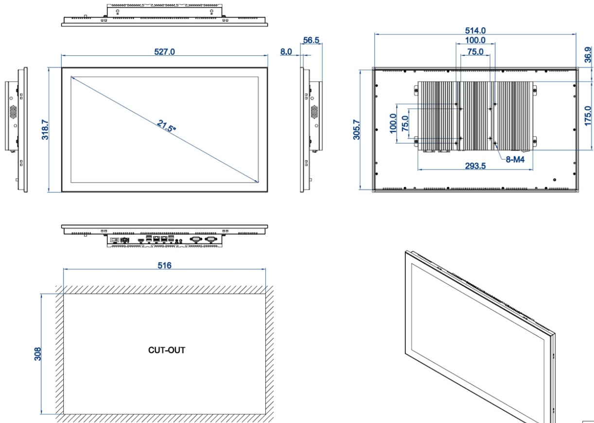
DIMENSIONAL DRAWING:TPC-DCM215
