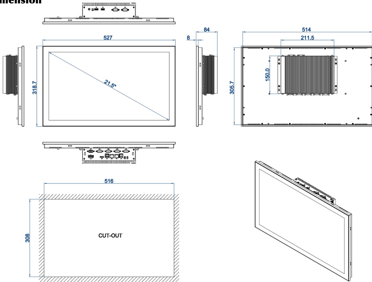
DIMENSIONAL DRAWING:TPC-PC215
