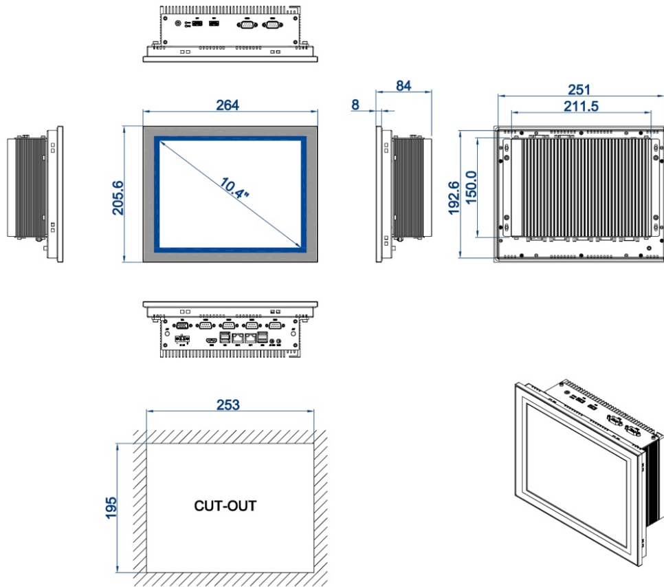
DIMENSIONAL DRAWING:TPC-PR104
