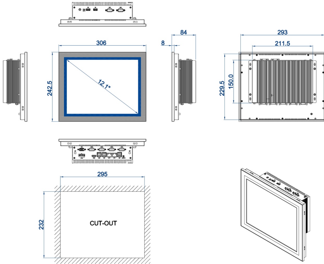
DIMENSIONAL DRAWING:TPC-PR121W
