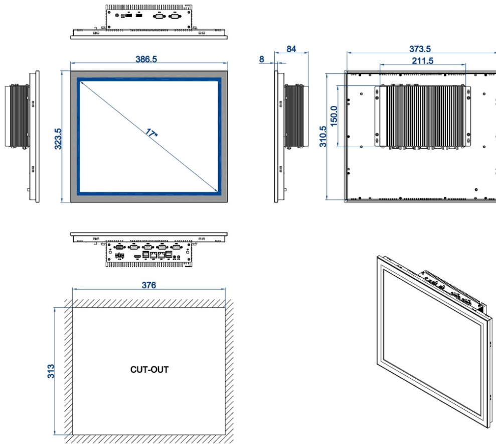
DIMENSIONAL DRAWING:TPC-PR170
