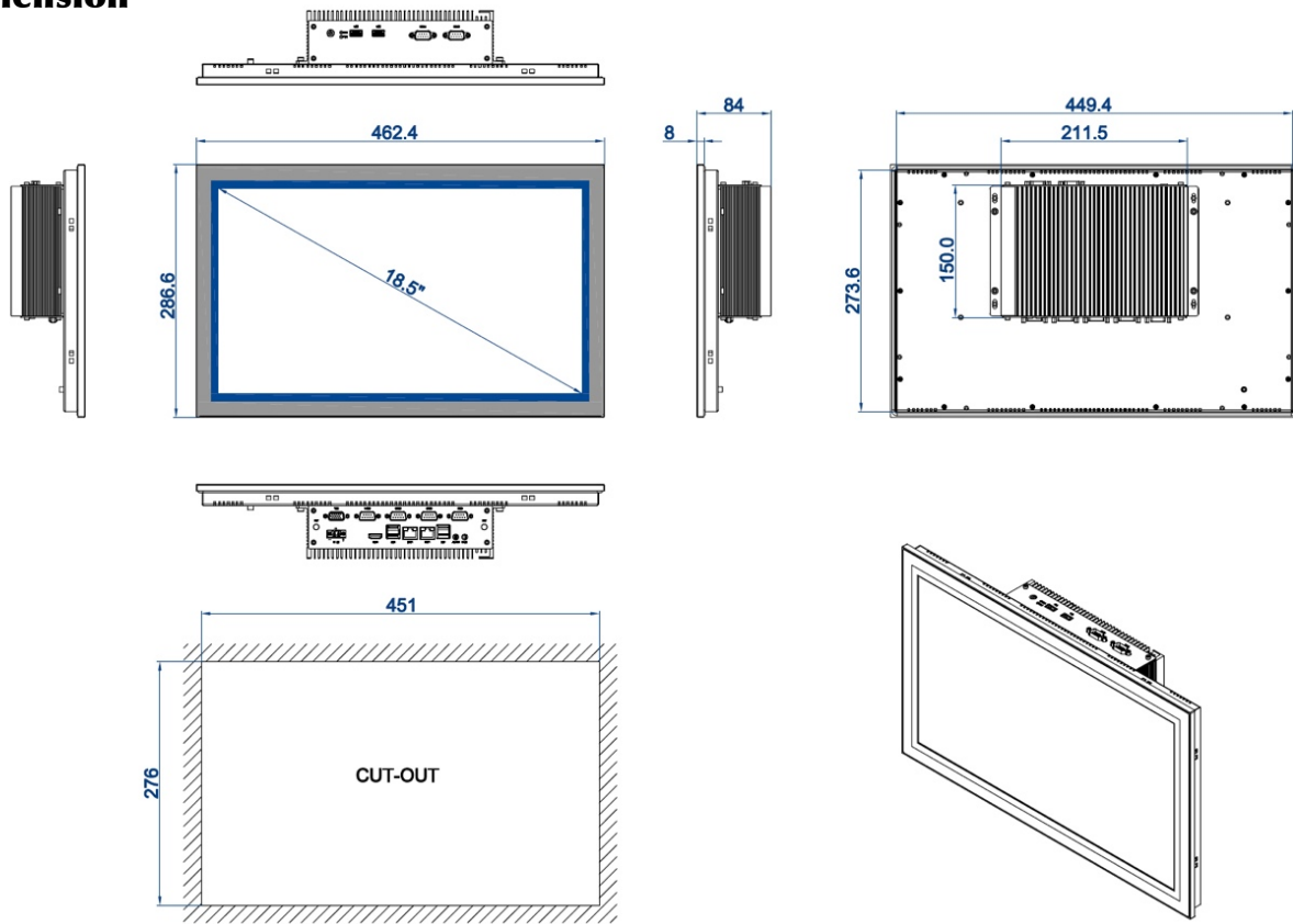
DIMENSIONAL DRAWING:TPC-PR185
