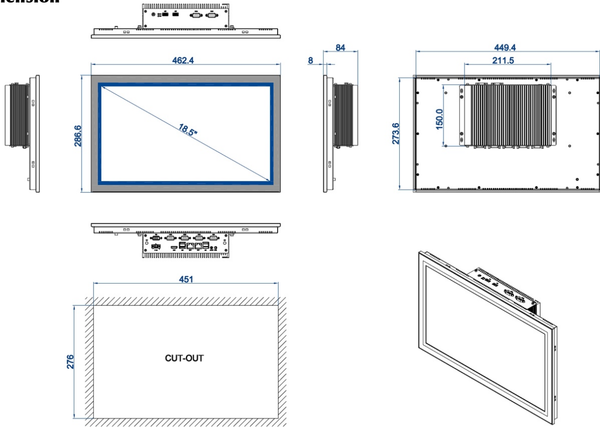
DIMENSIONAL DRAWING:TPC-PR185
