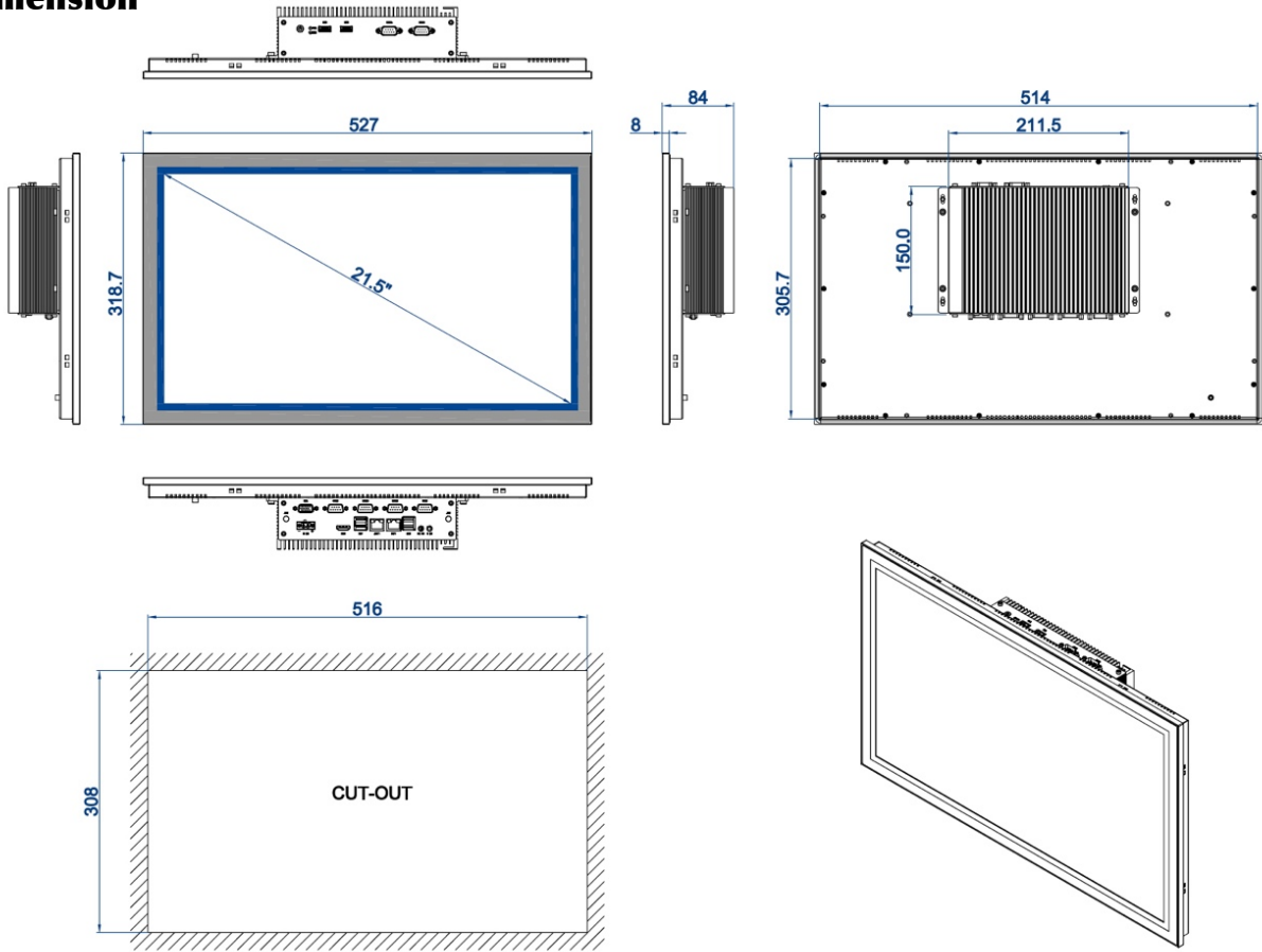
DIMENSIONAL DRAWING:TPC-PR215
