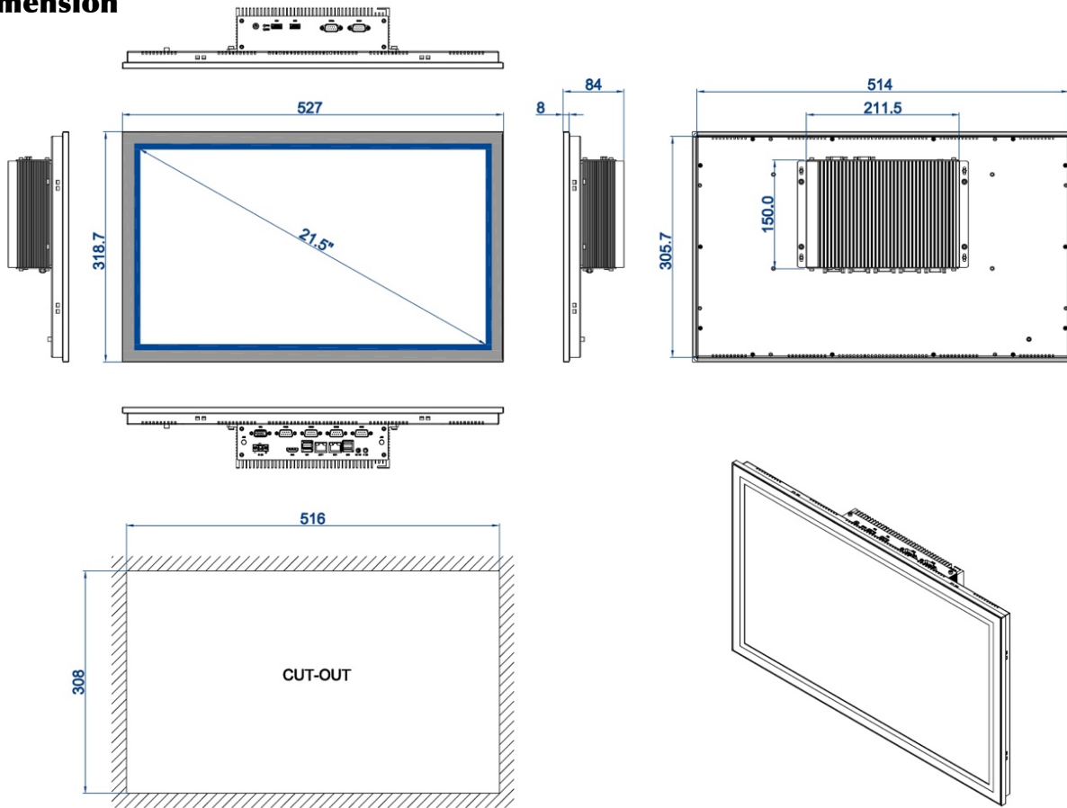
DIMENSIONAL DRAWING:TPC-PR215
