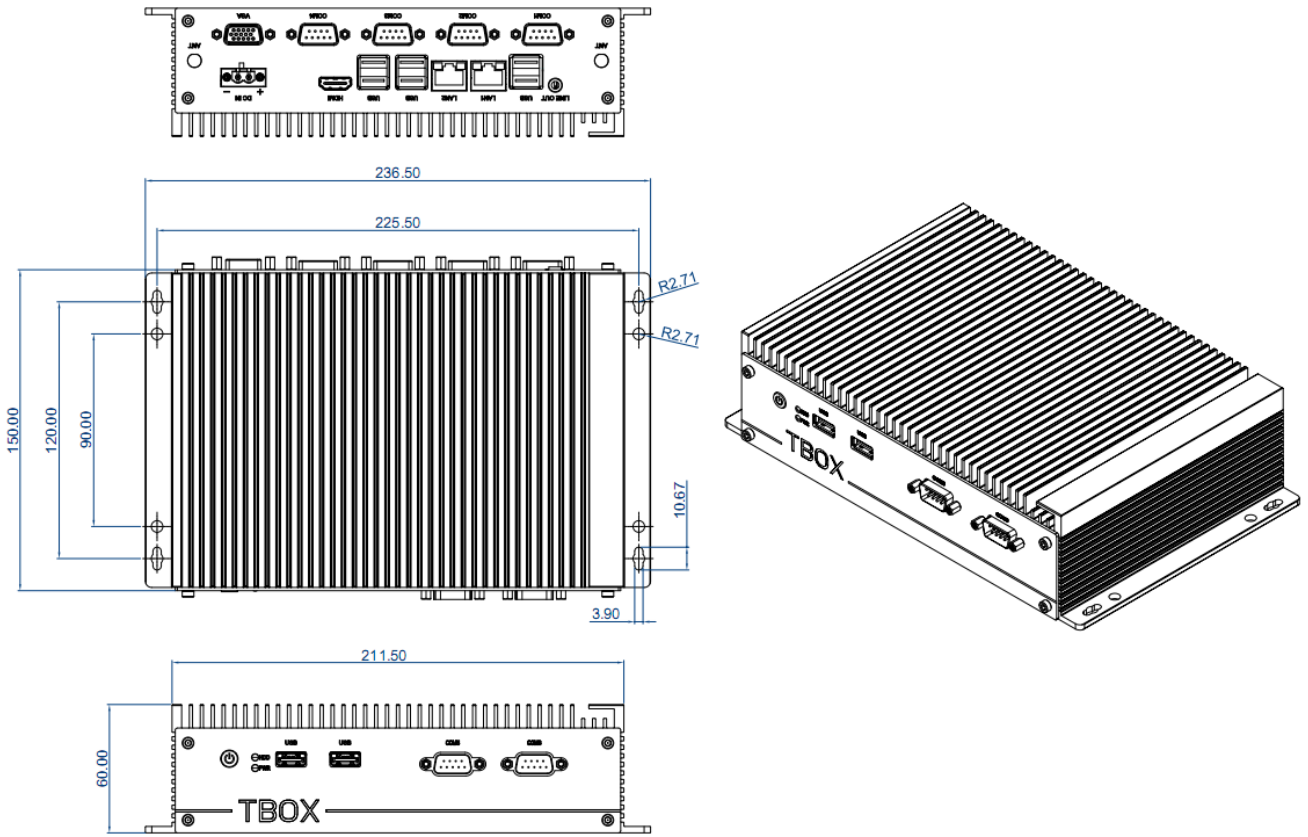
DIMENSIONAL DRAWING:TBOX-28X0
